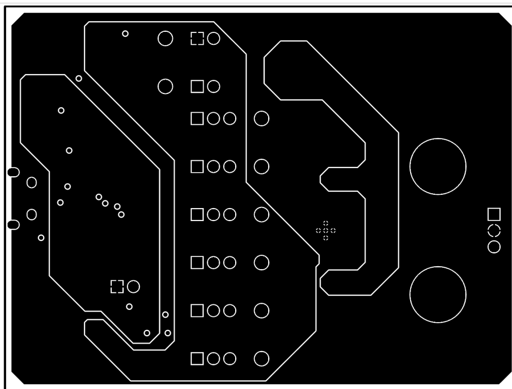
Figure 11. Signal Layer 2
