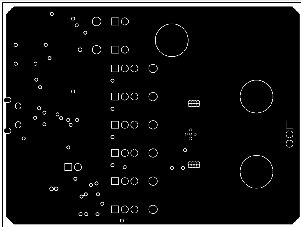
Figure 10. Signal Layer 1
