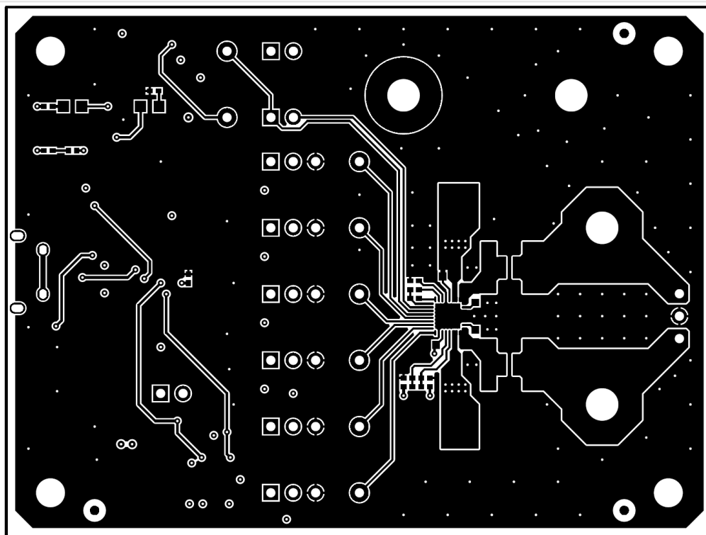
Figure 9. Top Layer
