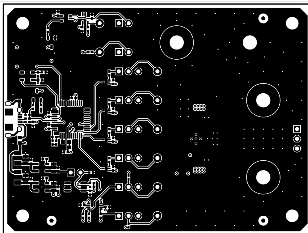
Figure 12. Bottom Layer
